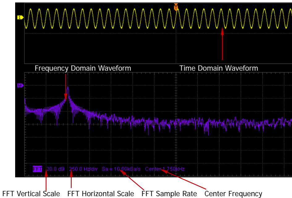
Figure 6-1 FFT Operation
