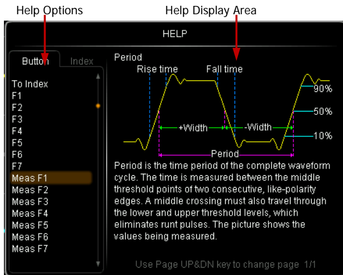
Figure 1-13 Help Interface
