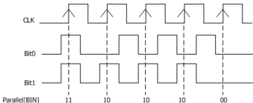
Figure 7-1 Parallel Decoding
